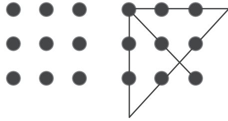
Fig. 24.2 The nine-dot problem. ( Left ) Subjects’ task is to draw four straight lines that go through all nine dots without backtracking or lifting the pencil from the paper. ( Right ) One solution to the problem.
